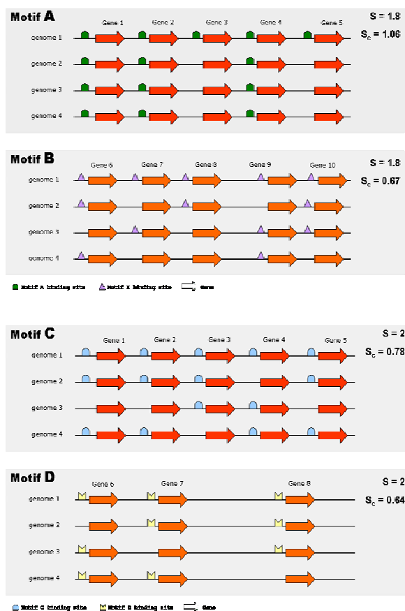
Figure 2. Shown are examples that highlight the differences between the conservation score, S , and the weighted conservation scores, S_c .
