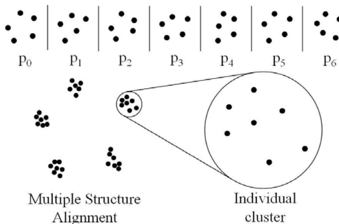
Fig. 1. Composite motif construction begins with the multiple structure alignment of the individual motifs p_0, p_1 , etc, yielding clusters of correlated points in the ultimate alignment. We describe this iterative alignment process in Section 3.2.
