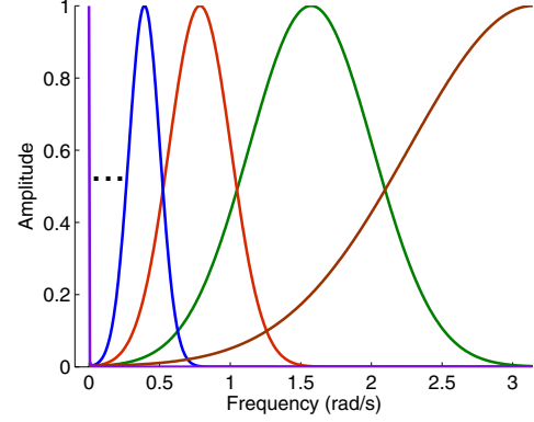
Fig. 4. Frequency supports of the non-uniform Gabor filters.
