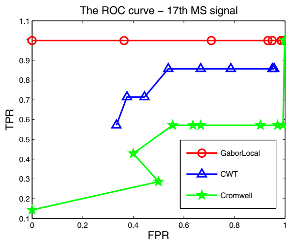
Fig. 14. The ROC curve of three methods such as Cromwell, CWT, and our method with the 17 th mass spectrum signal
