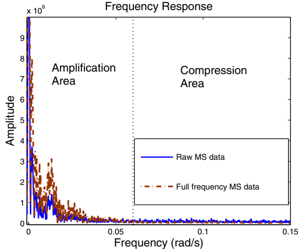
Fig. 9. The frequency response of the 19 th MS signal of CAMDA 2006 before and after using the summary filter.
