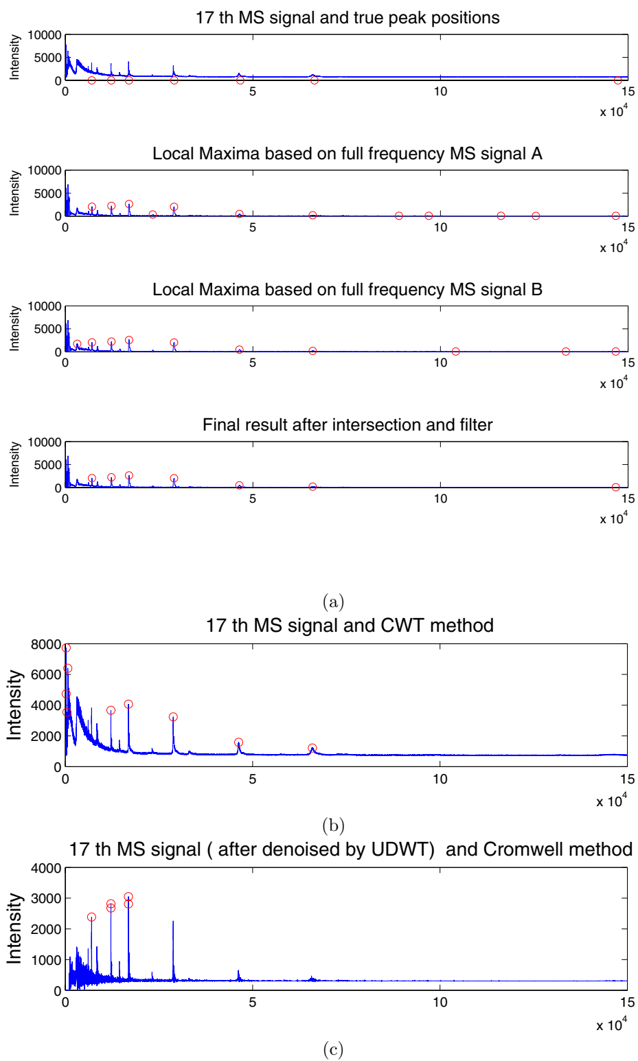
Fig. 15. Example of peak detection of the 17 th mass spectrum signal using (a) our GaborLocal method, (b) CWT method, and (c) Cromwell method.
